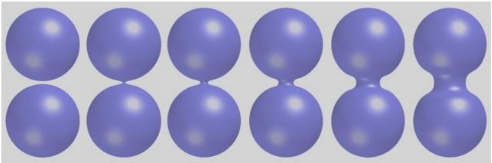
Figure 1: Sequence of the coalescence process of two droplets
